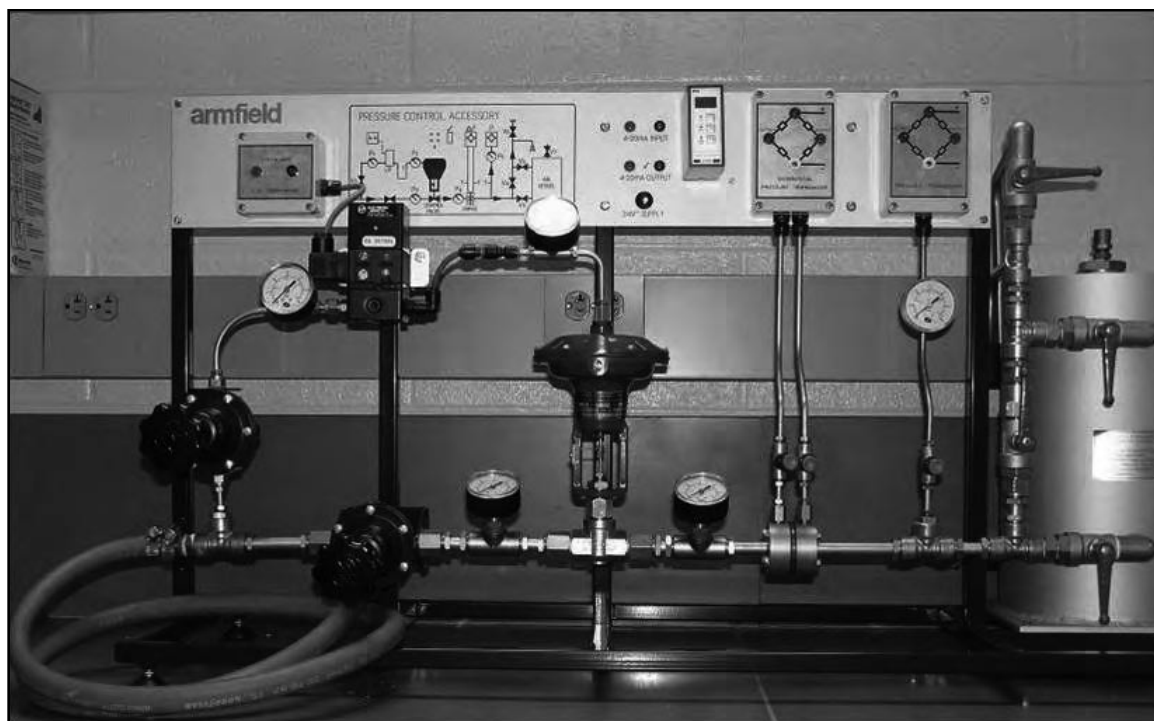
Figure 2. (below right) Control panel for pressure regulation apparatus.
